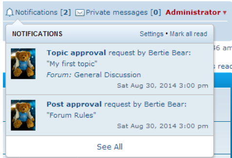
Figure 5.4. Notifications Menu
