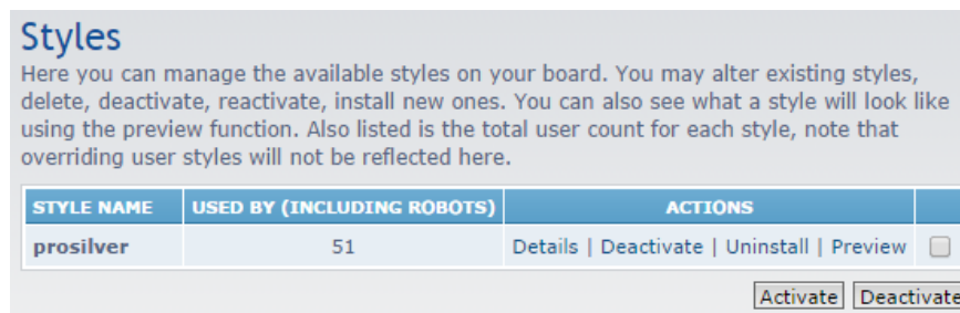
Figure 3.8. Styles overview
